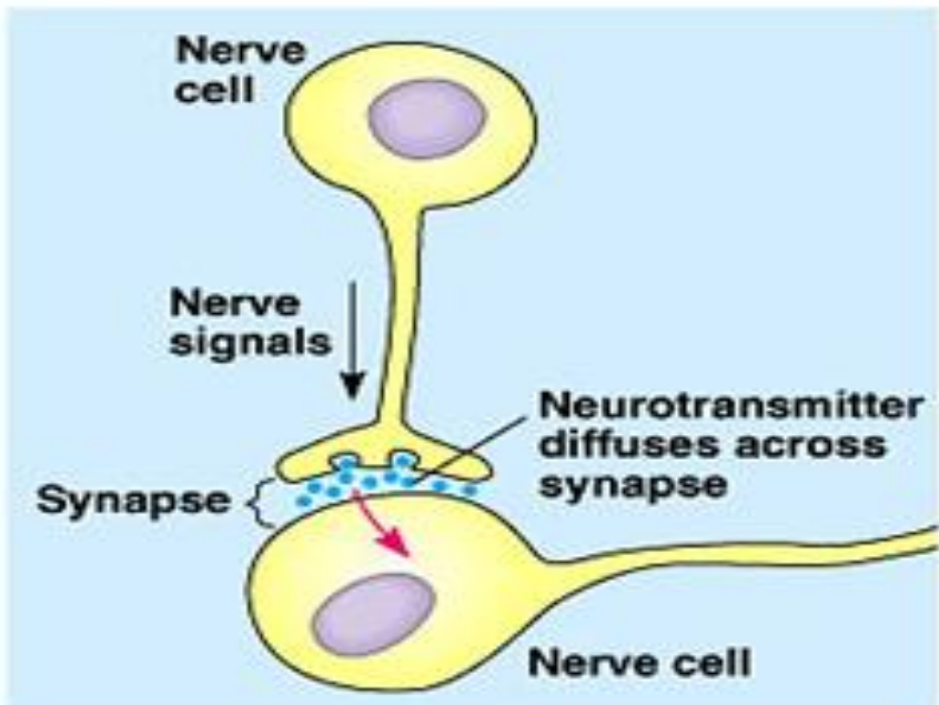
Synaptic signaling
